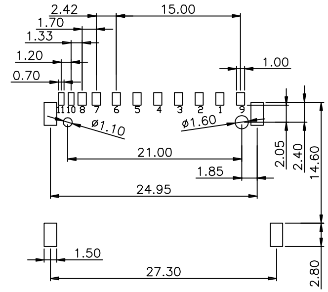
PCB LAYOUT
