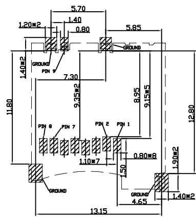
RECOMMENDED PCB LAYOUT (ALL TOLERANCE ARE ±0.05)
